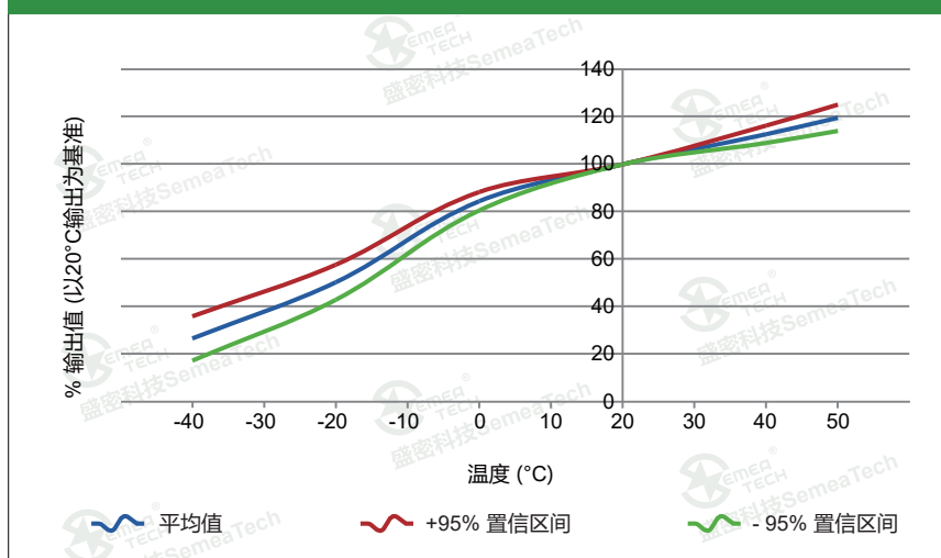
盛密科技 Commercial CO-1000C 传感器温度性能
